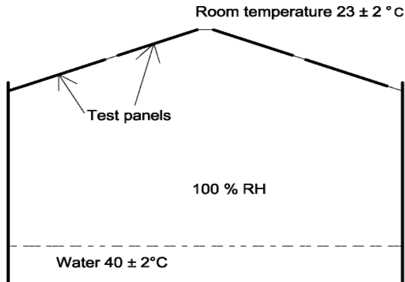
Figure 3 : Condensation chamber (1/7/2006)
