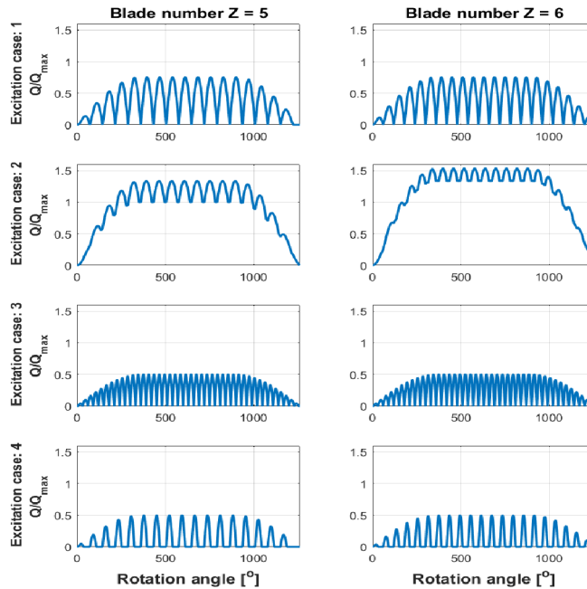
Figure 5 : The shape of the propeller ice torque excitation sequences for propellers with 5 and 6 blades (1/7/2020)
