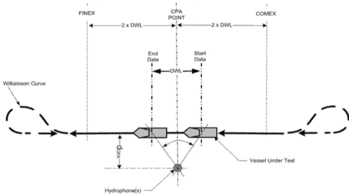
Figure 3 : Test course configuration (1/3/2017)
