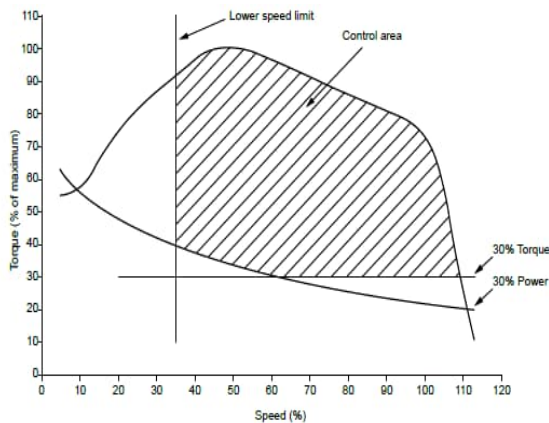
Figure 1 : Control area for variable speed auxiliary engines (1/7/2023)
